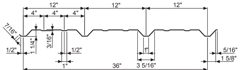
Reverse R-Panel Cross Section
