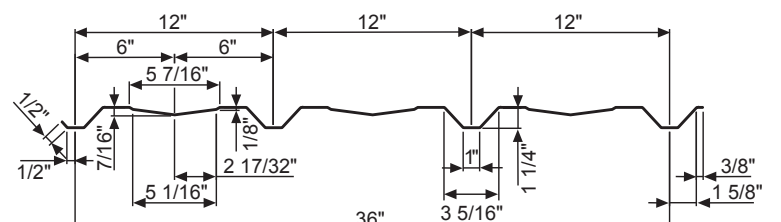
A-Panel Cross Section
